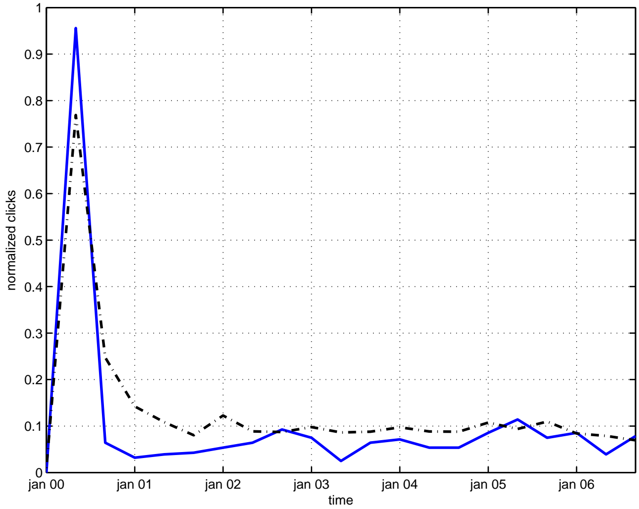
violation statistics
