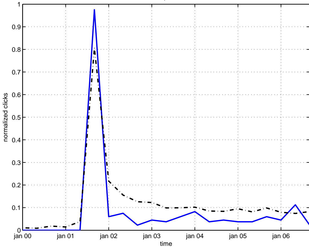
violation planck law
