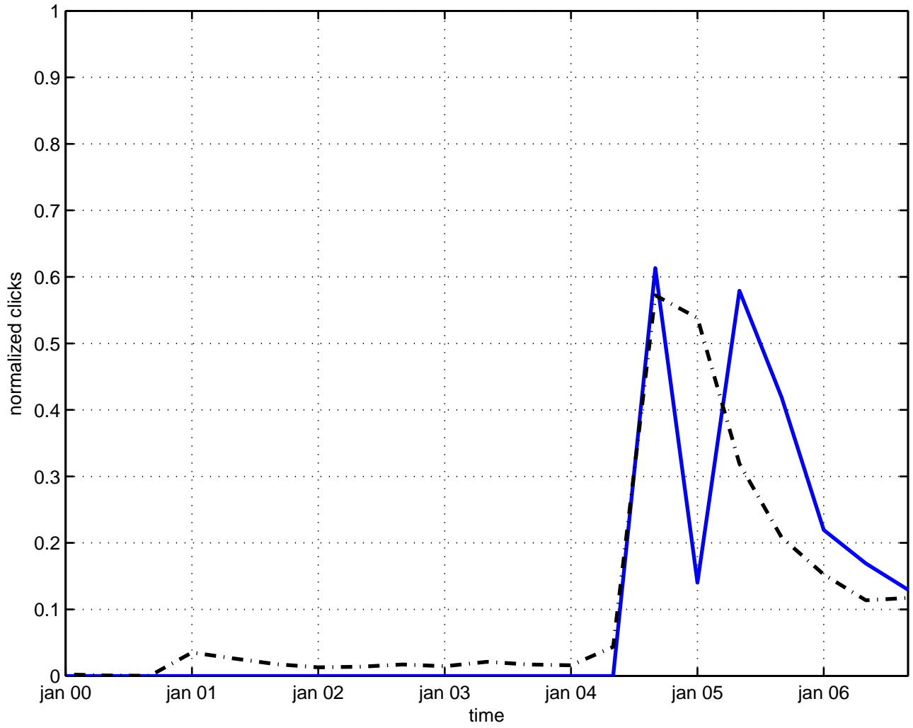
violation pauli principle
