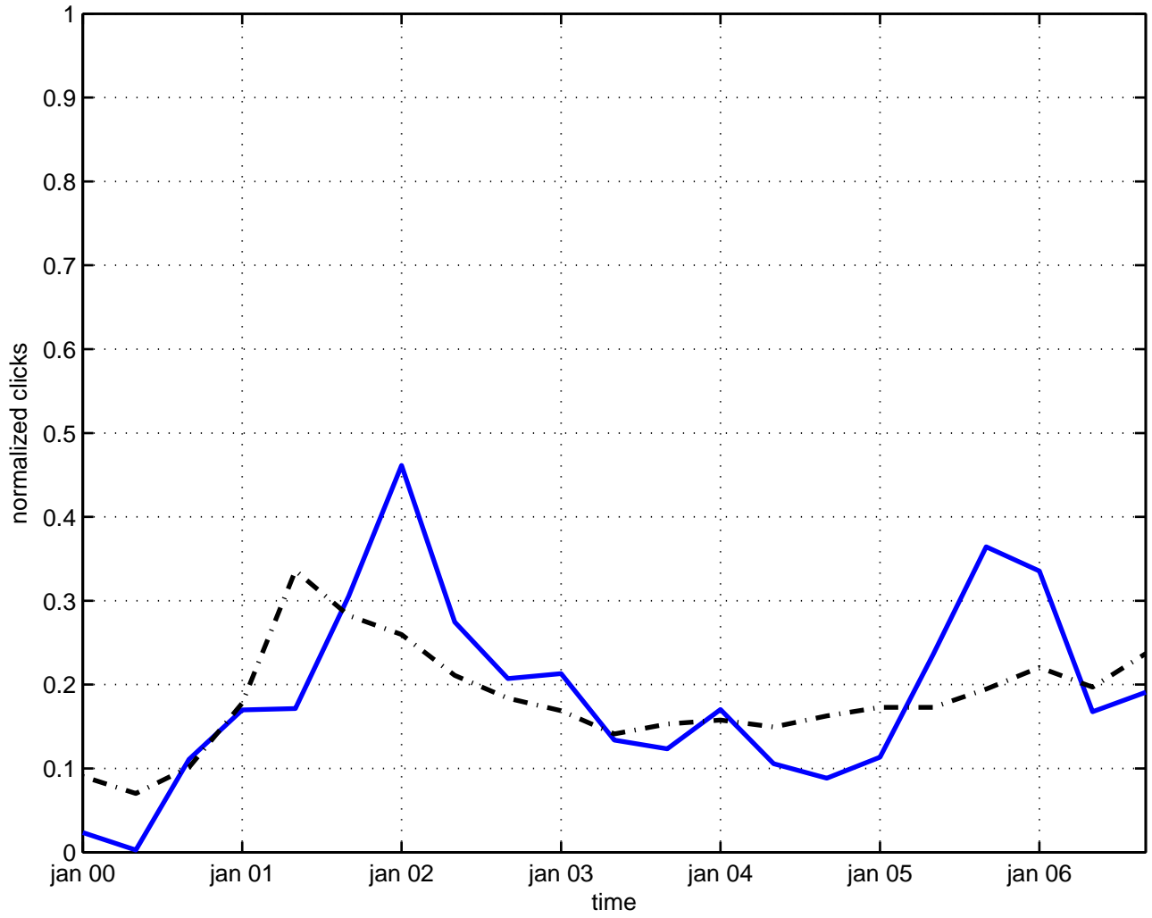
violation parity
