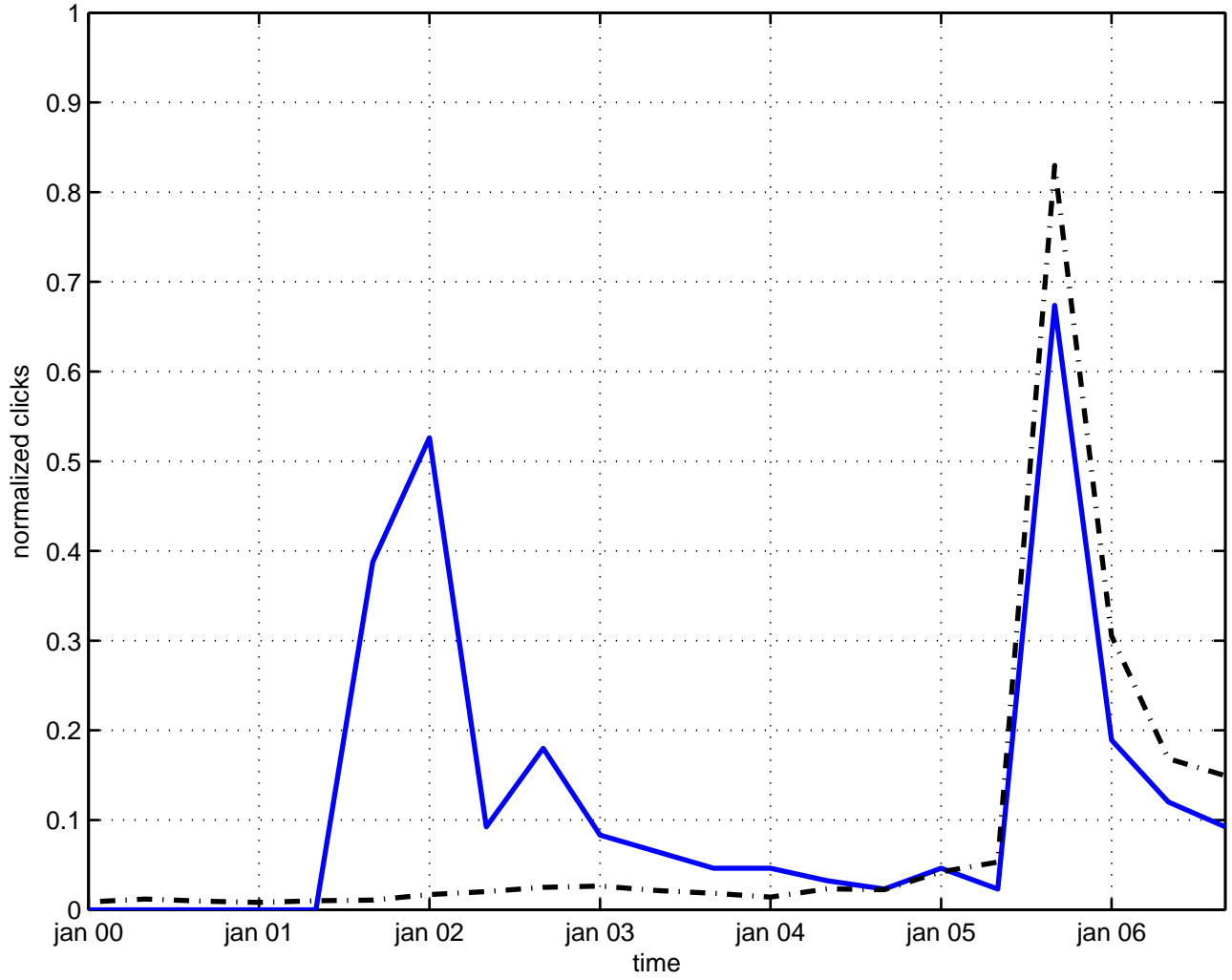
violation fermion number
