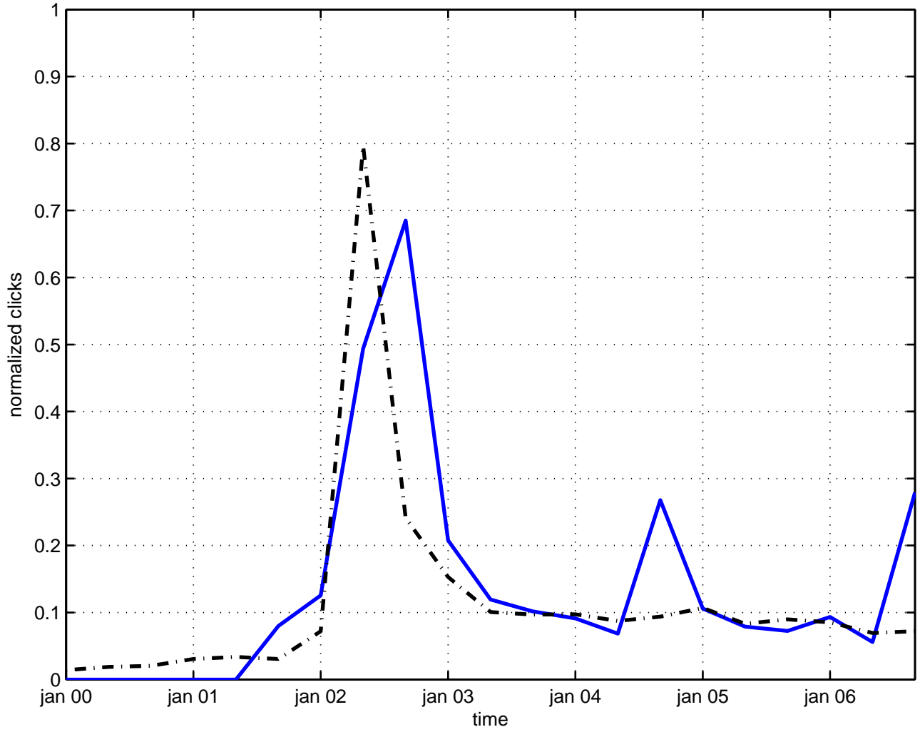
violation equivalence principle
