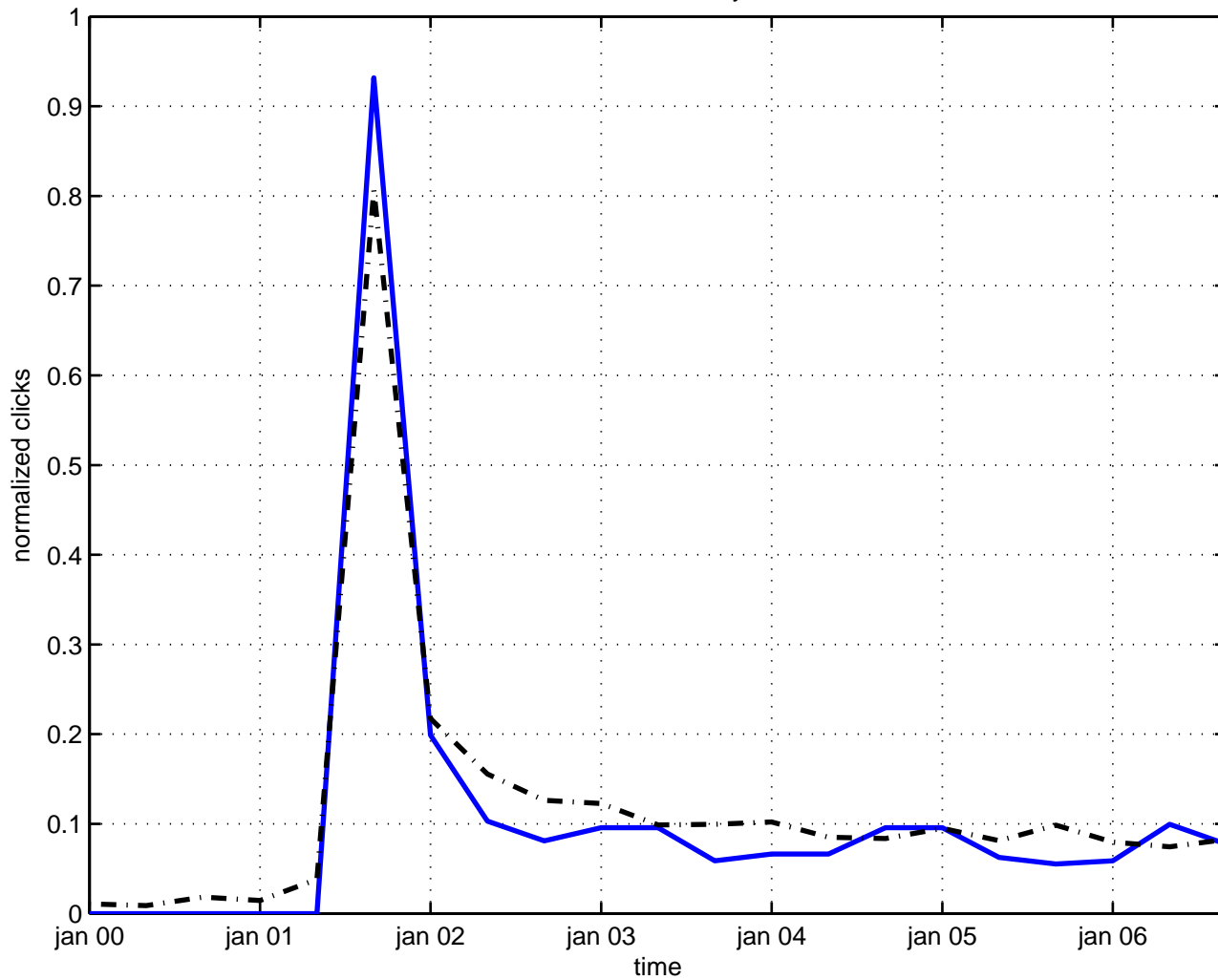
violation duality
