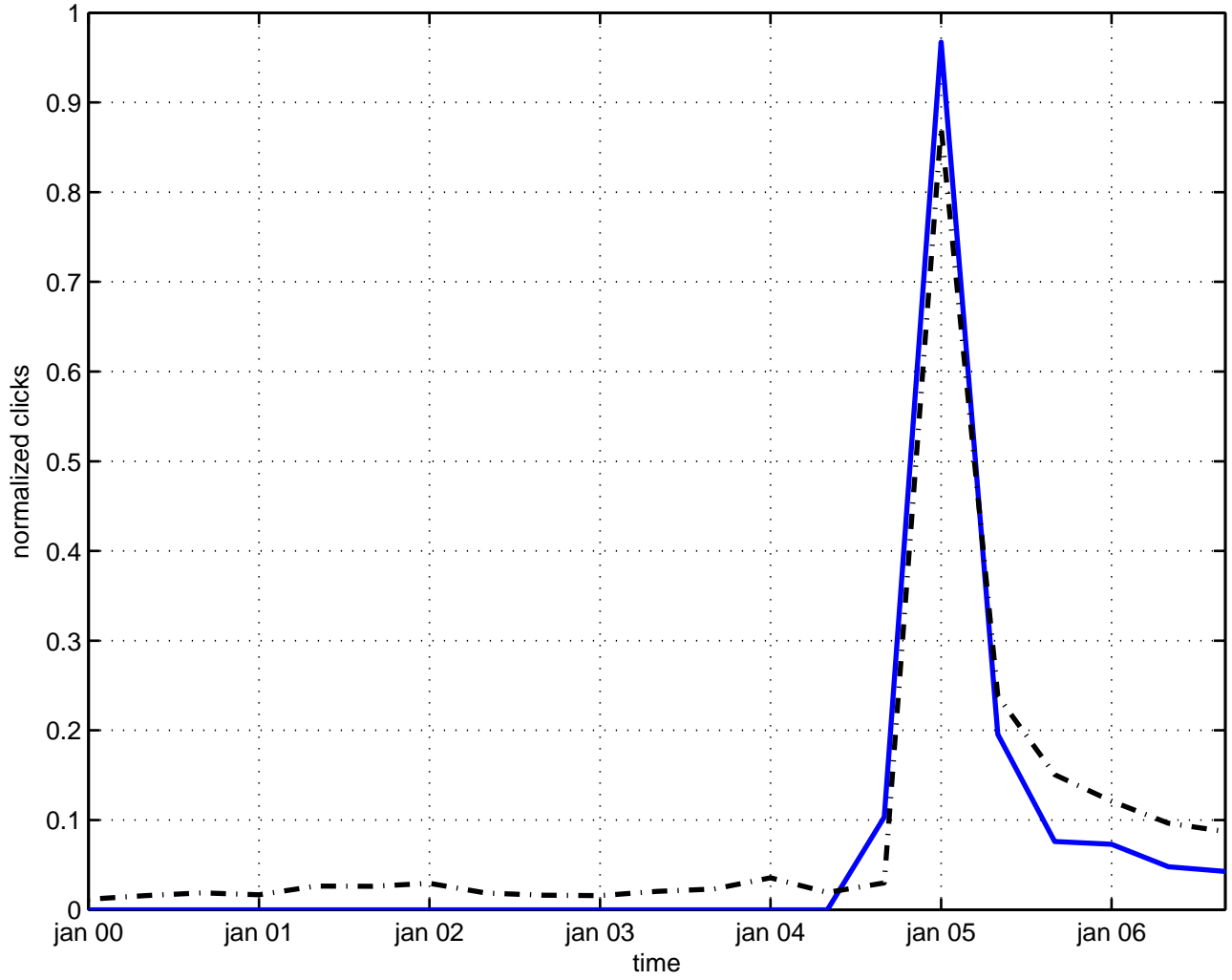
violation diffeomorphism
