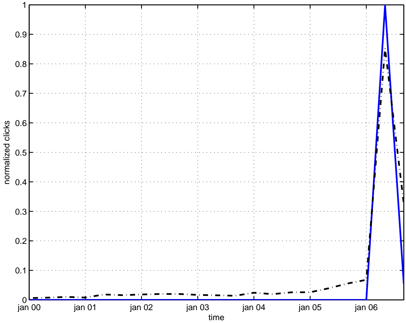
violation bell inequality
