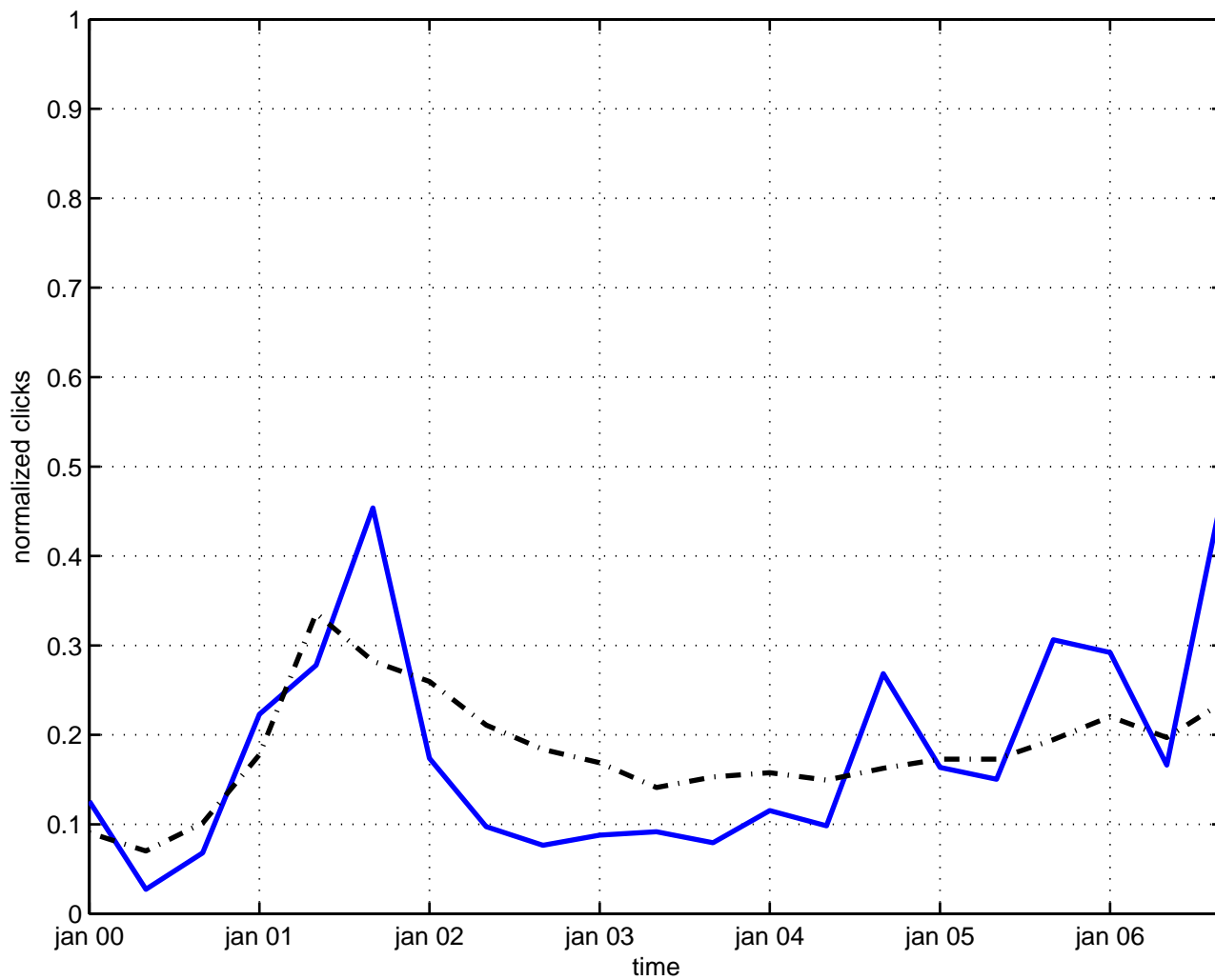
vertex model
