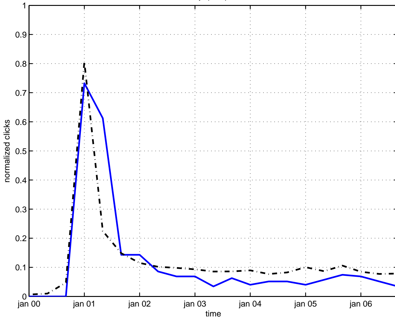
velocity quasiparticle
