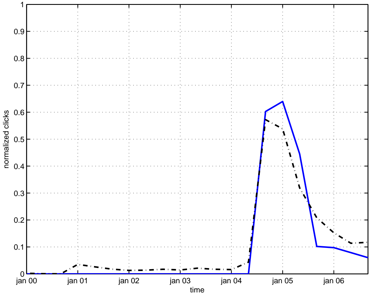
velocity neutrino
