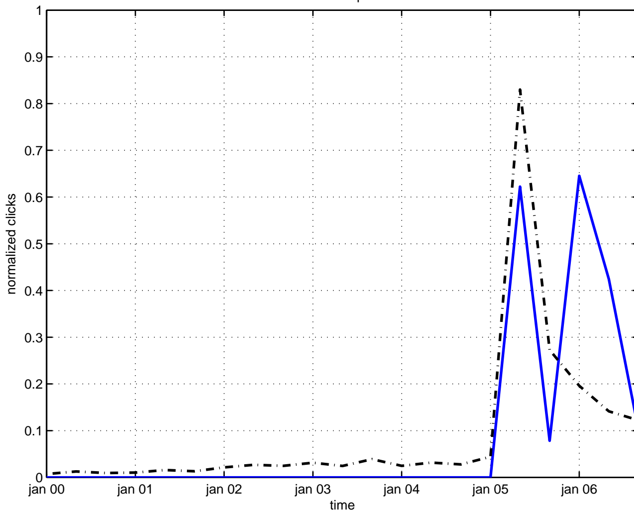
vector spin
