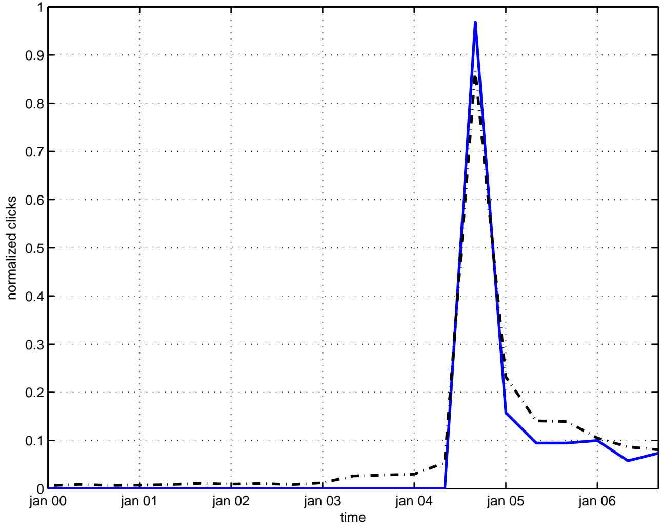
vector space
