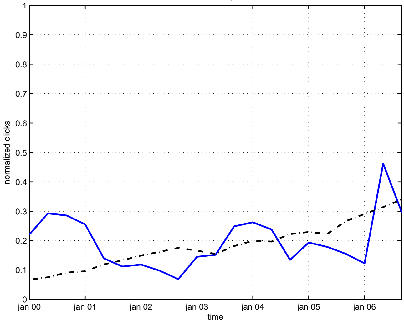
vector multiplet
