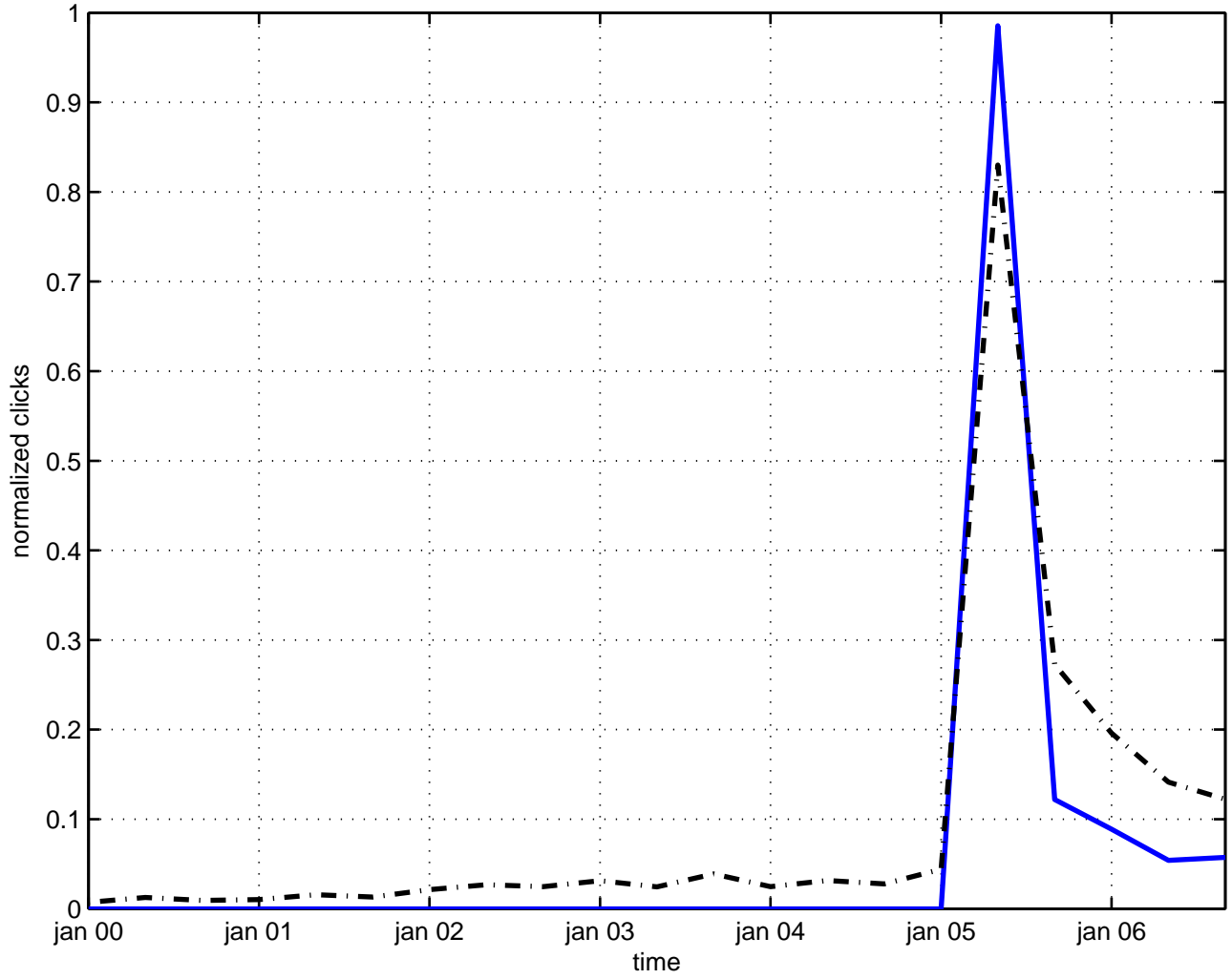
vector condensation
