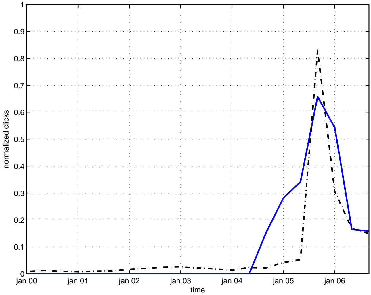
varying speed of light
