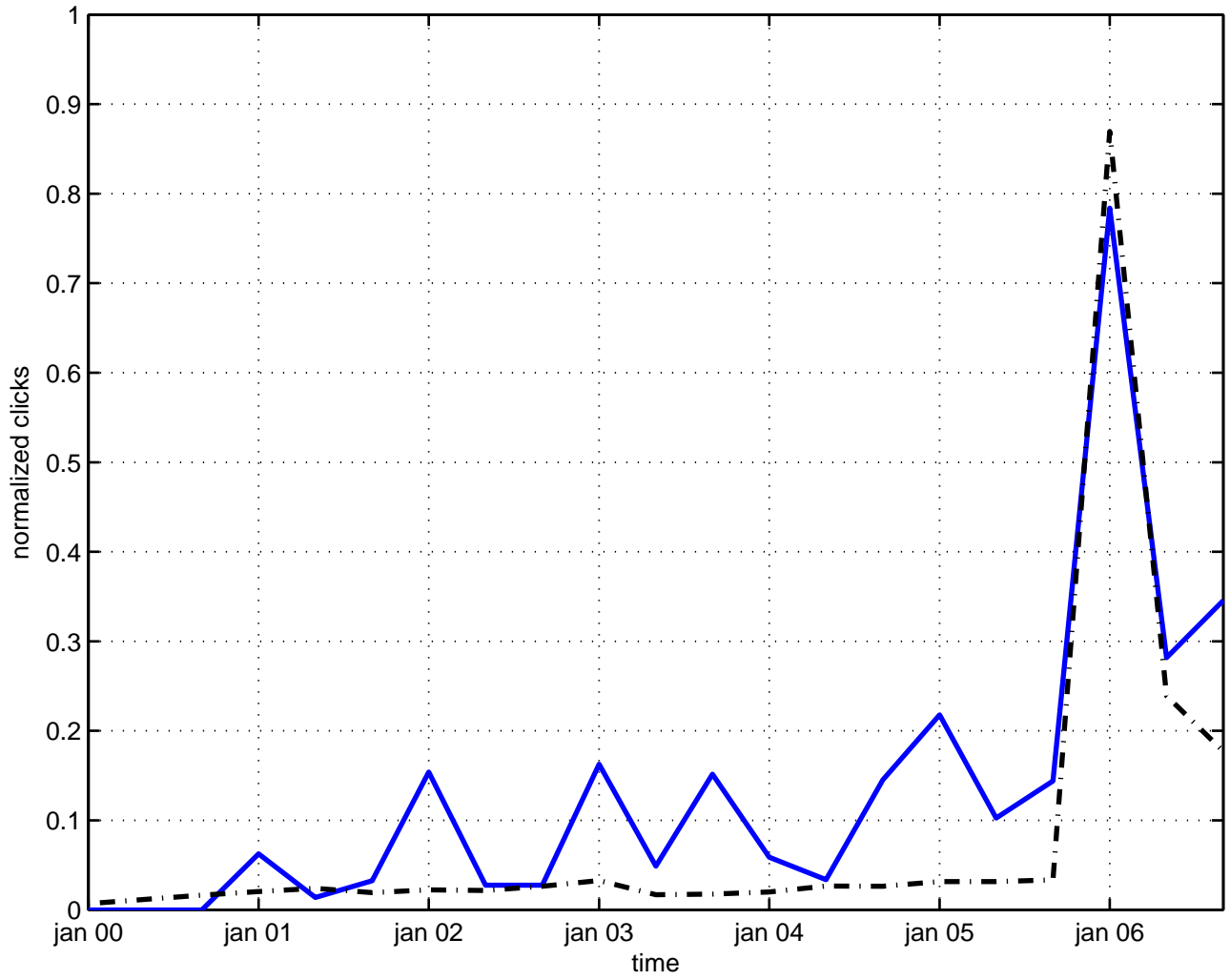
variational
