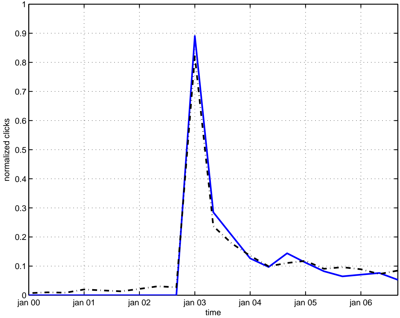
variational perturbation theory
