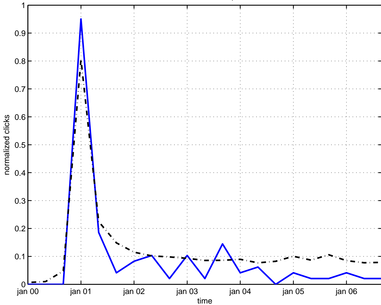
variational cumulant expansion
