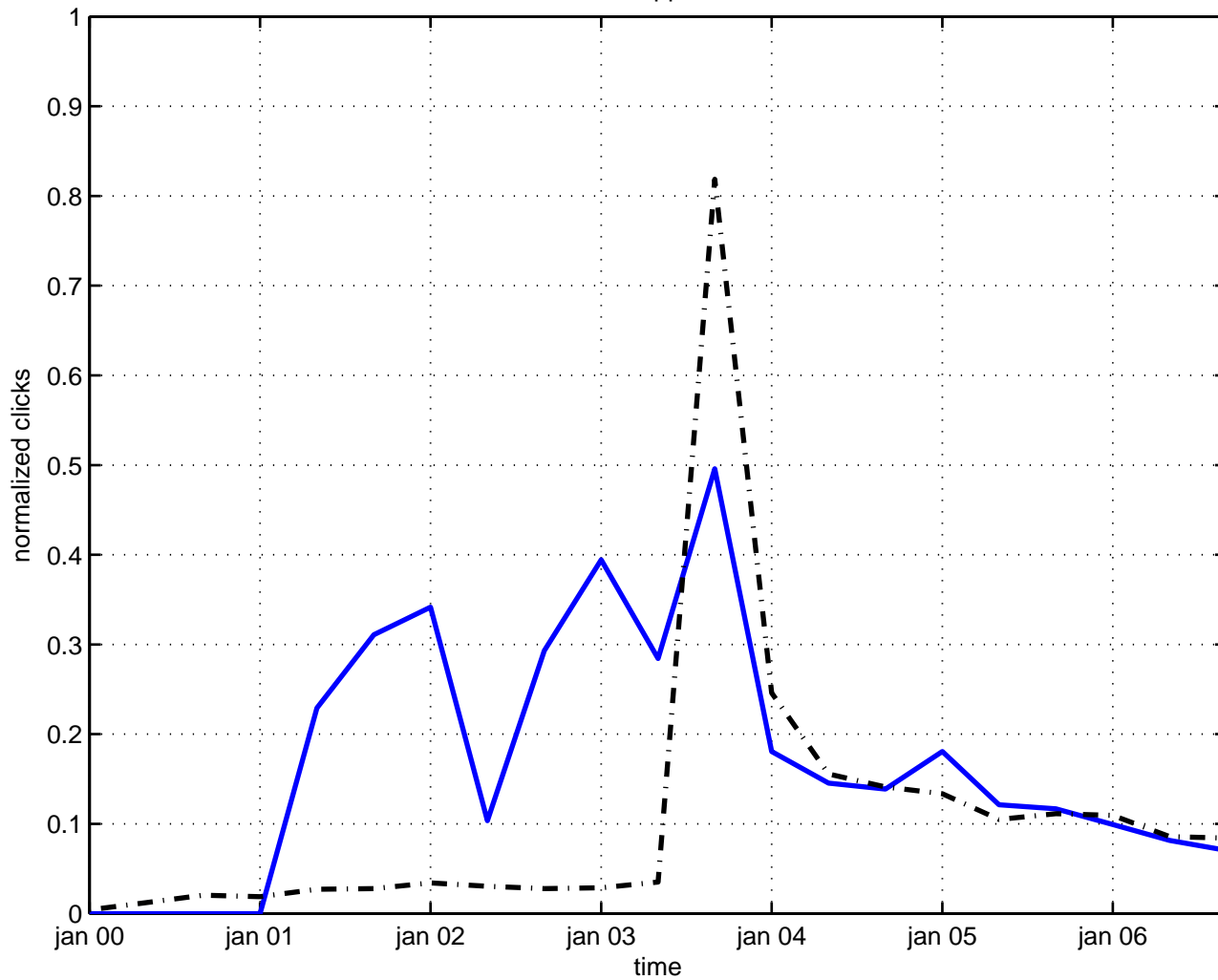
variational approximation
