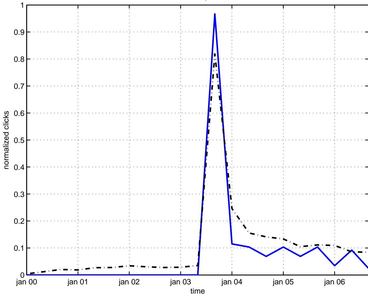
valence quark
