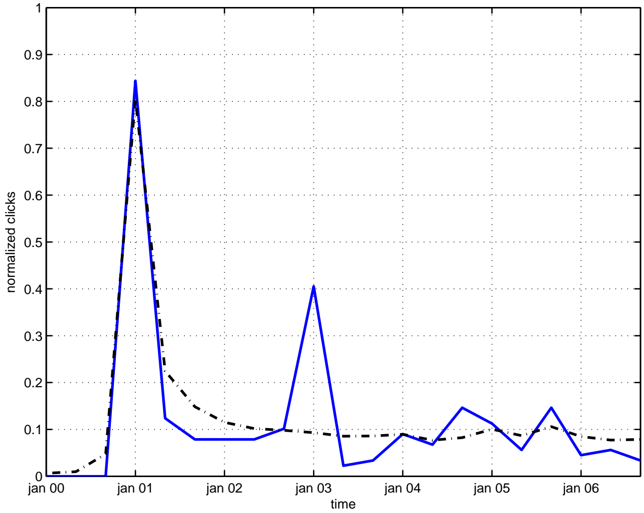
valence gluon
