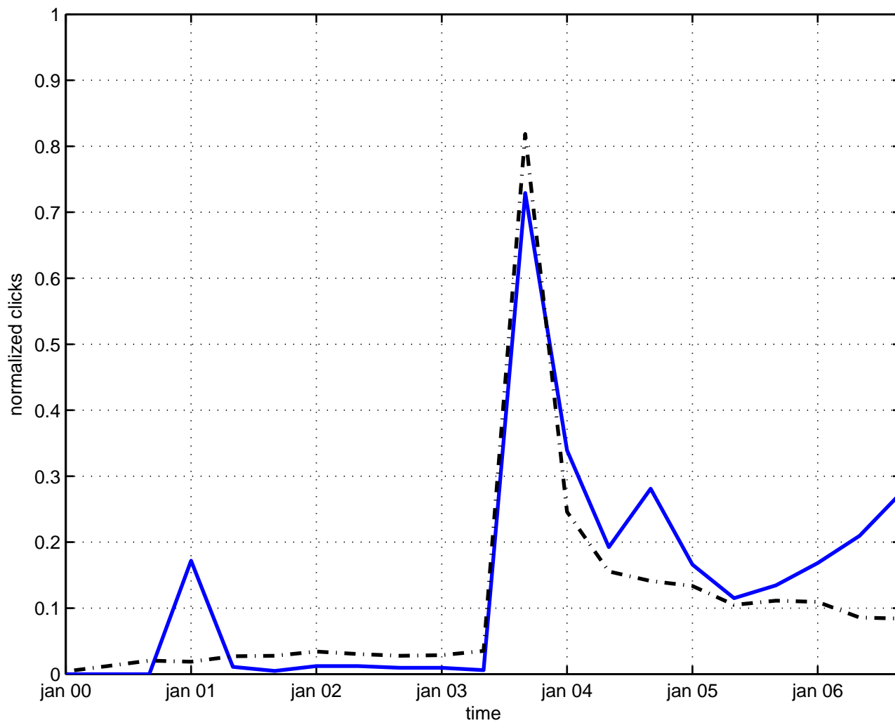
vafa-witten theorem
