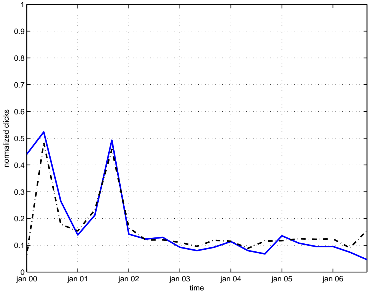
vacuum state quantum chromodynamics
