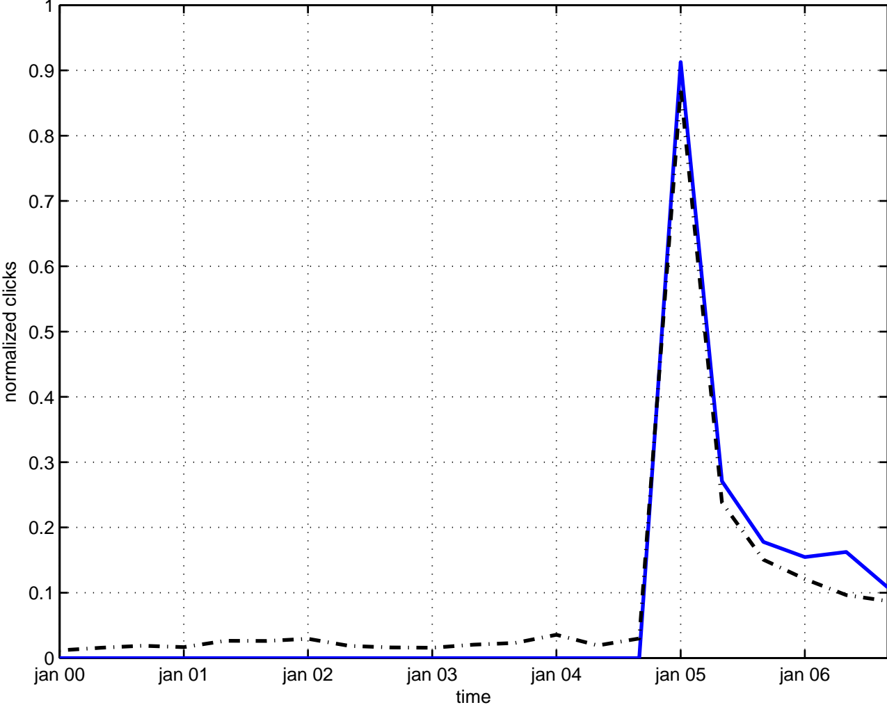
vacuum state ghost
