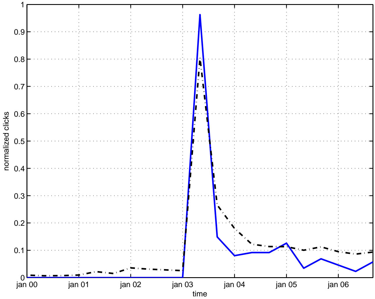
vacuum polarization star
