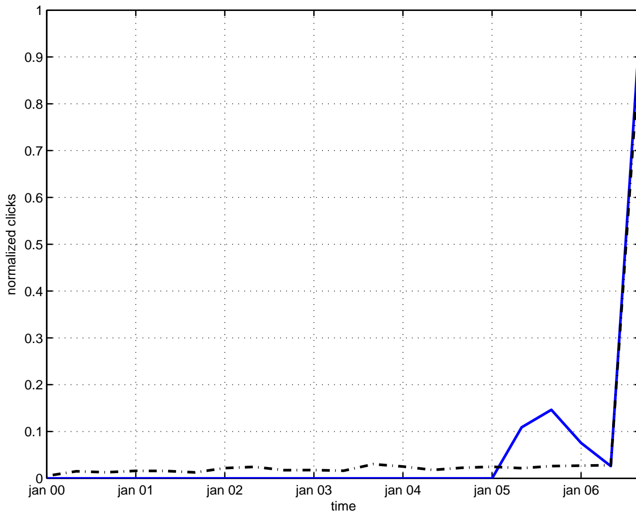
vacuum fluctuation
