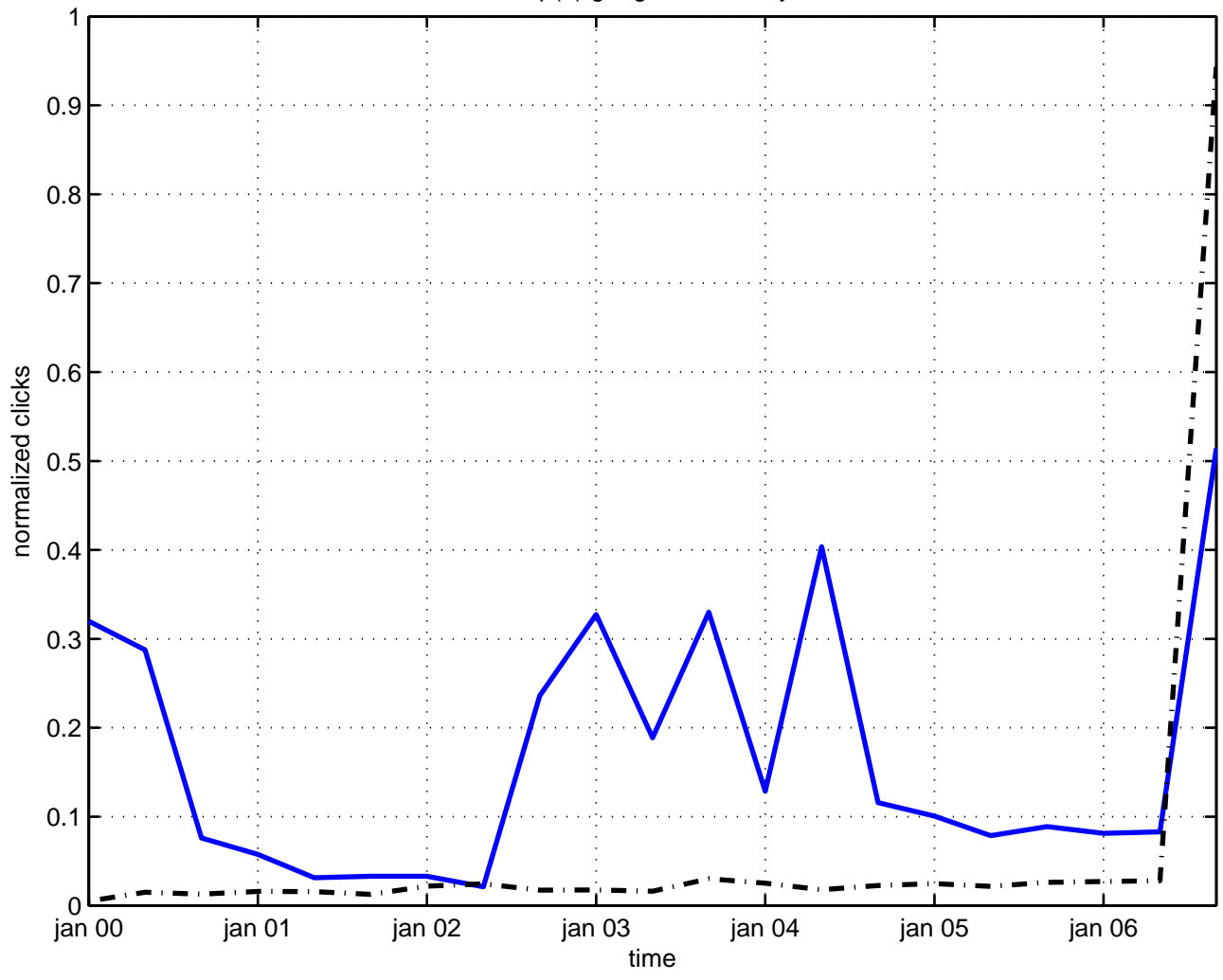
usp(n) gauge field theory
