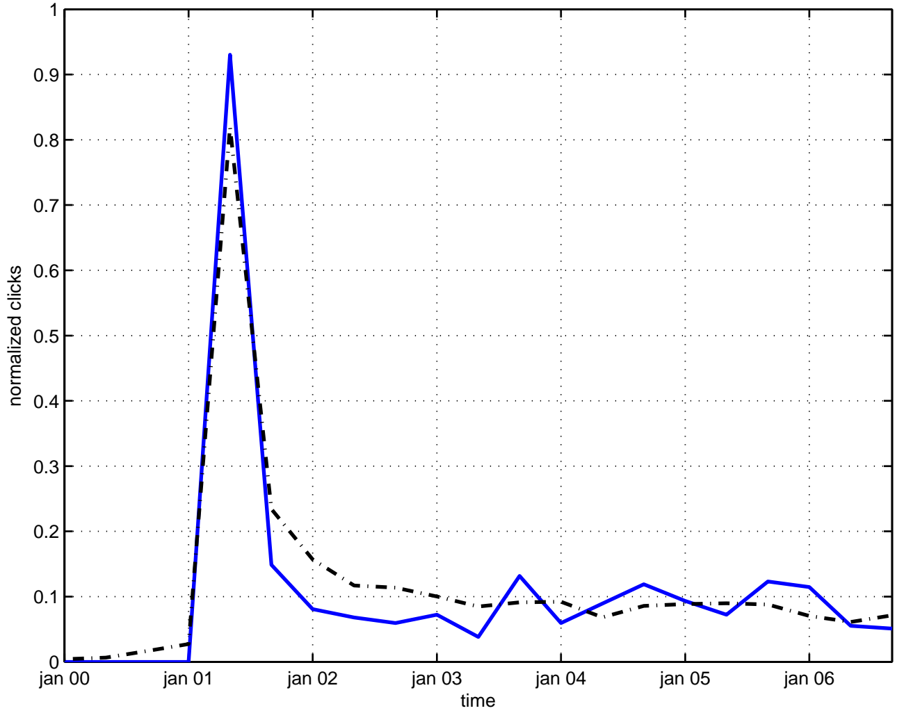
upper limit entropy
