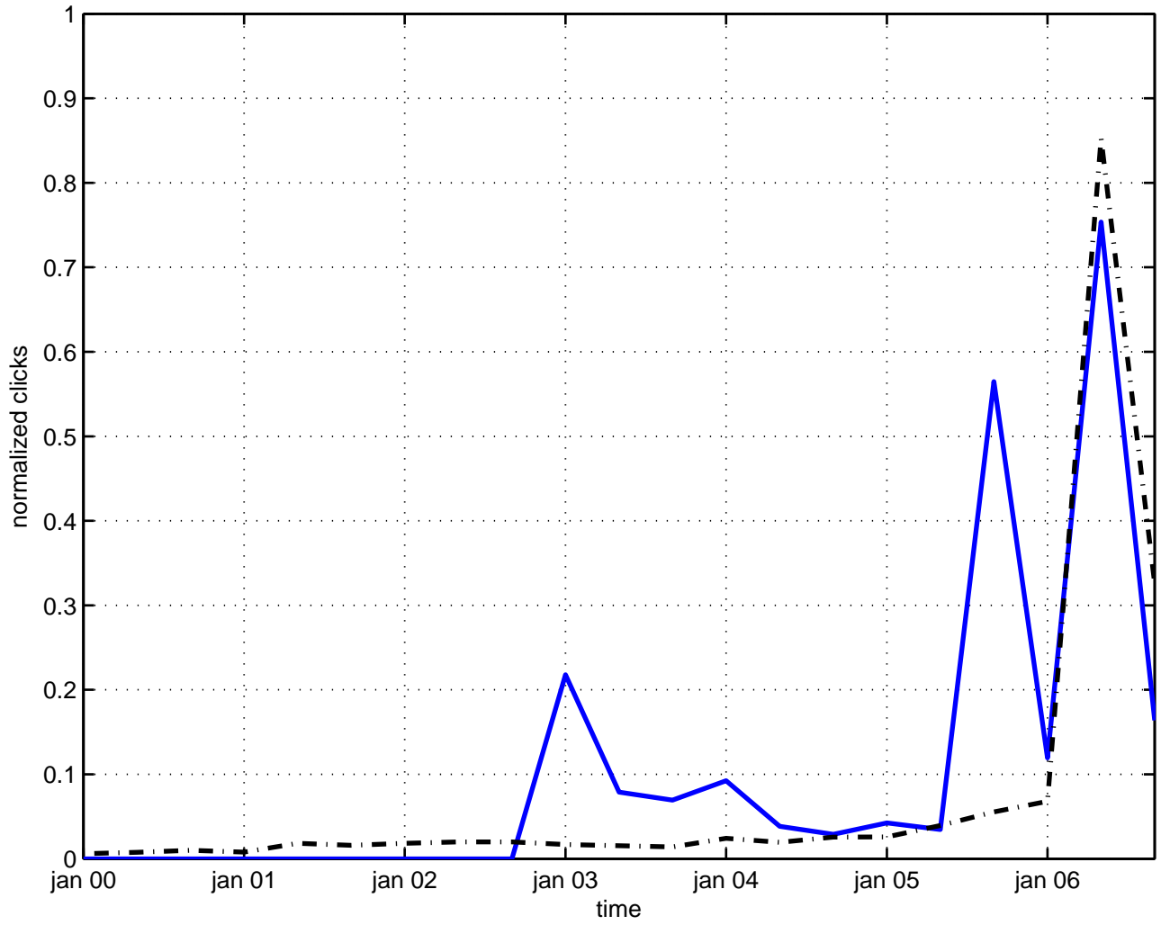
unruh radiation
