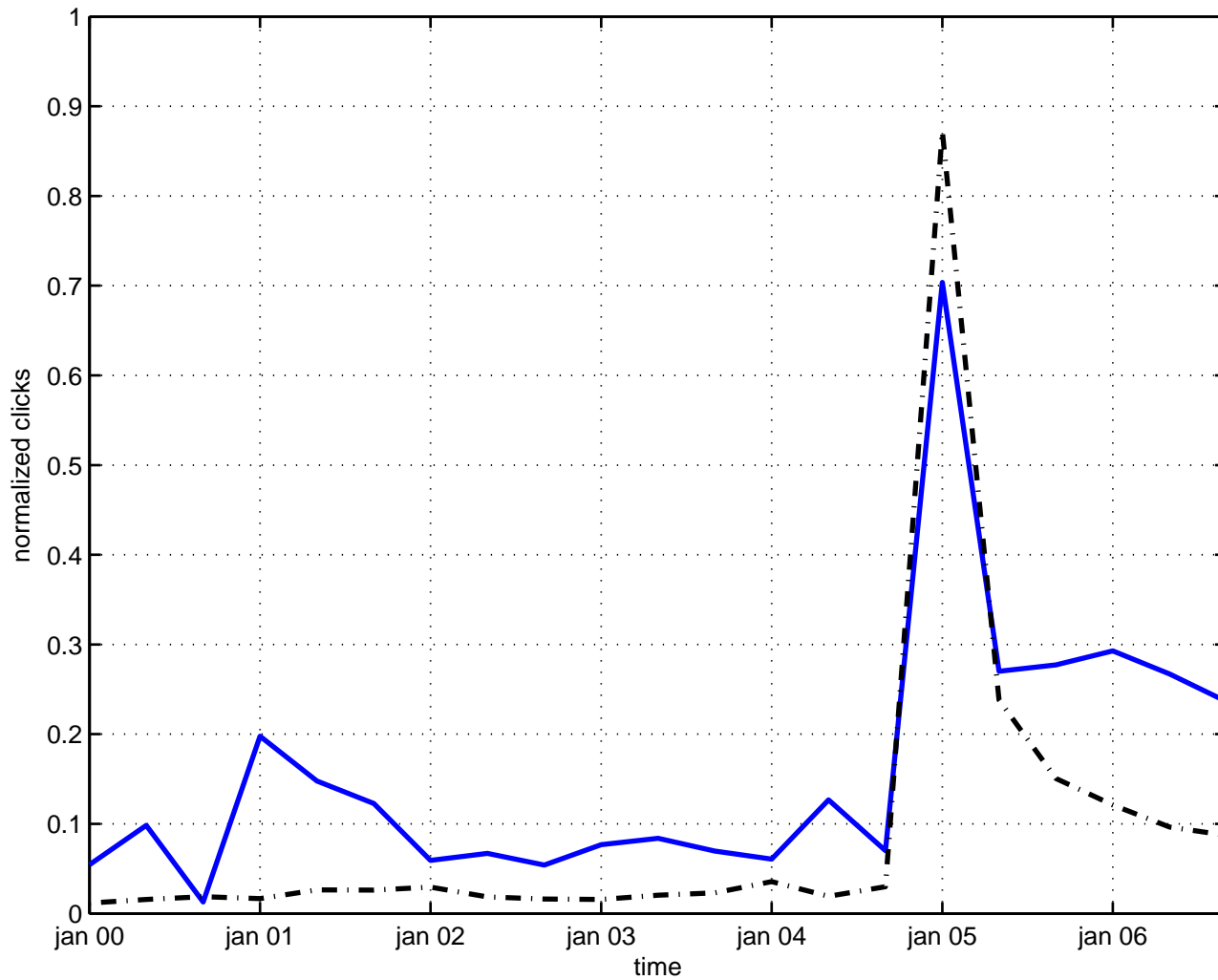
unruh effect
