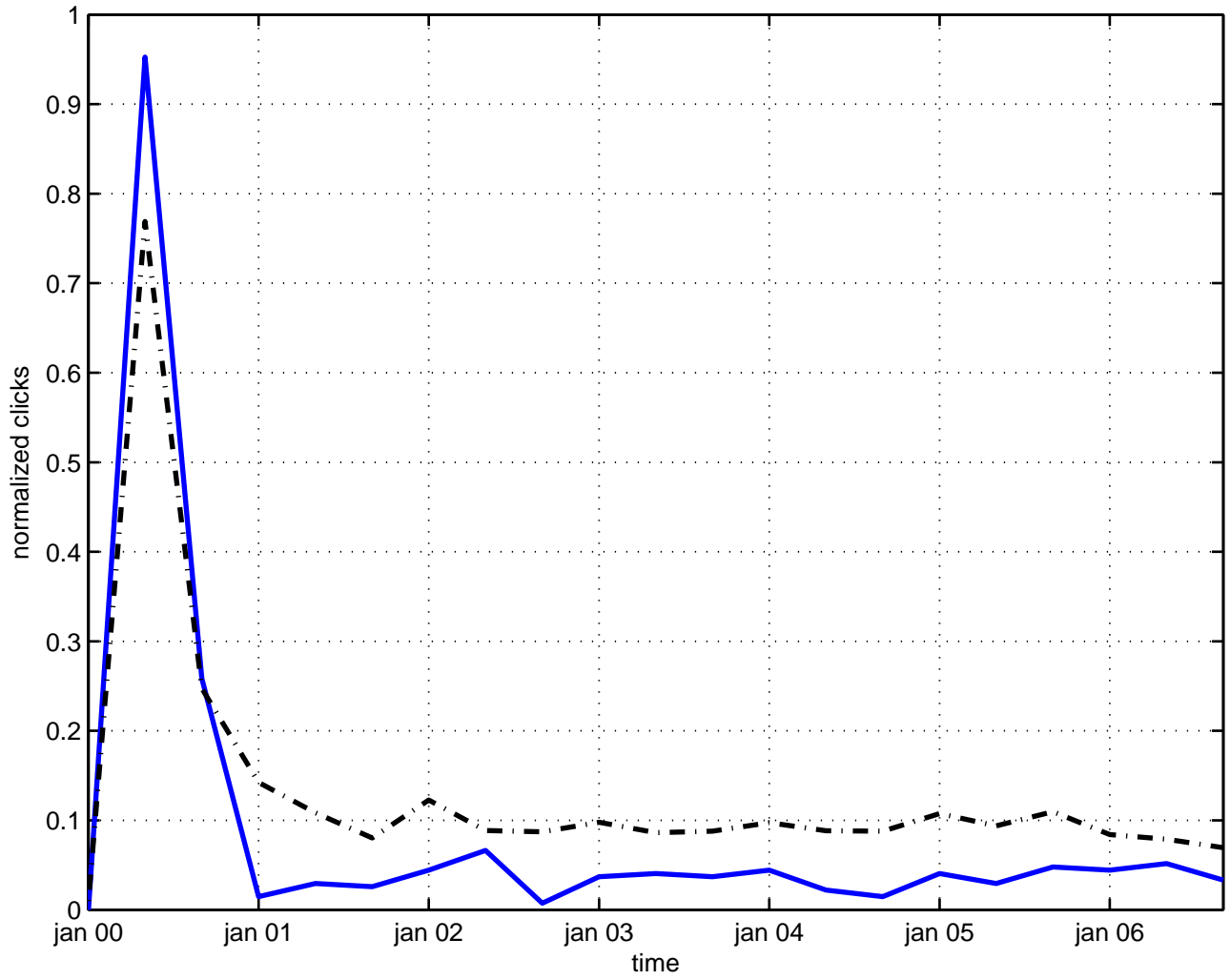
universality string model
