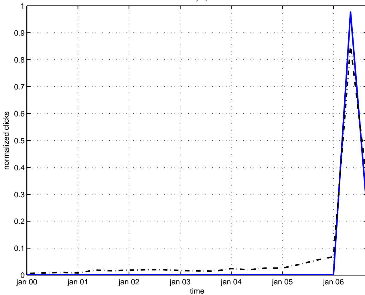
universality spectrum
