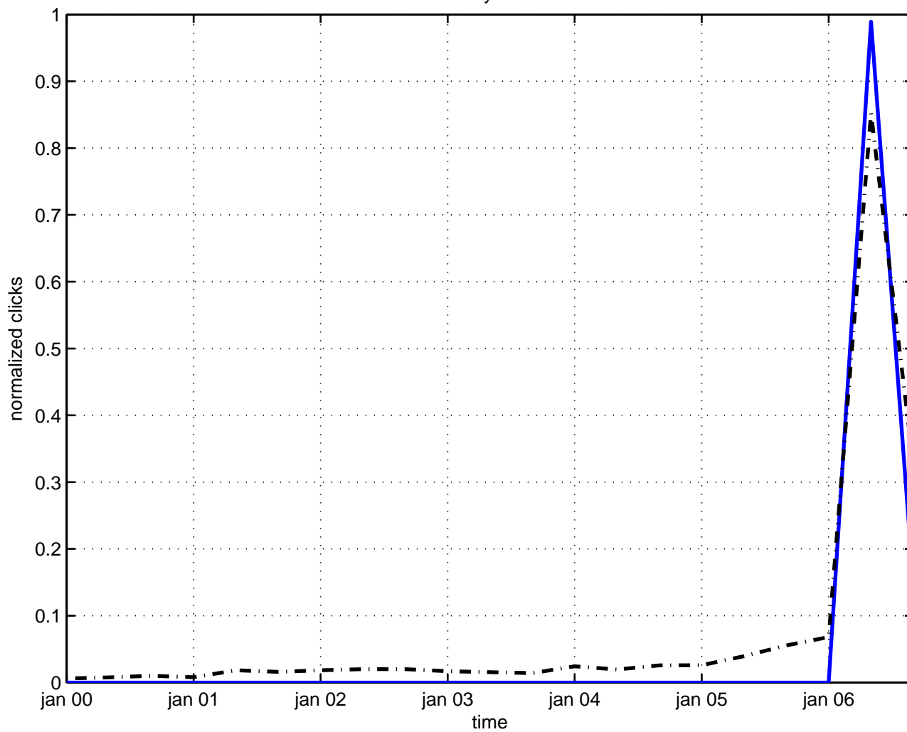
universality correction
