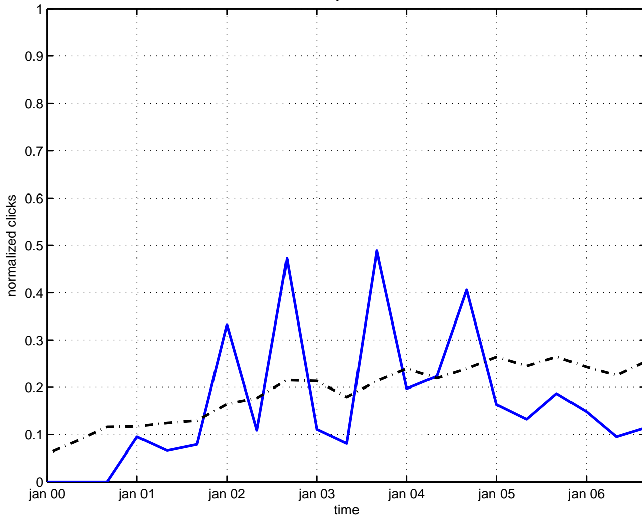
unitarity s-matrix
