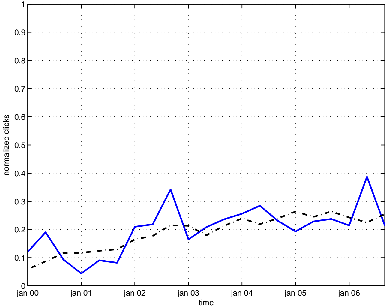
uncertainty relations
