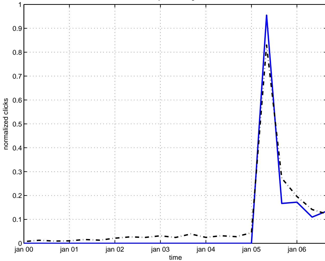
uncertainty relations gravitation
