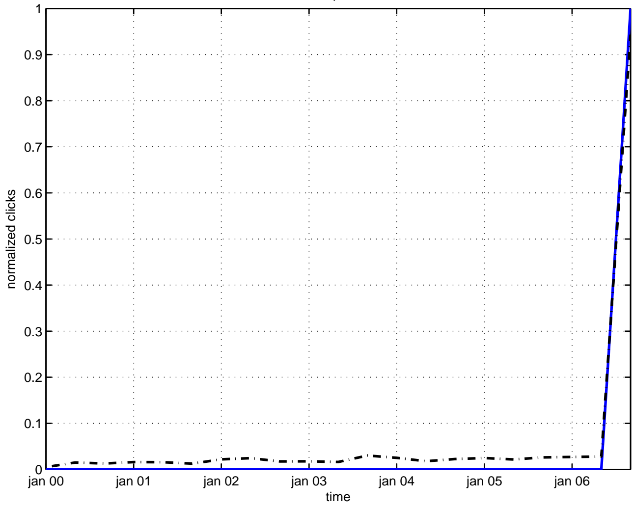
ultraviolet perturbation
