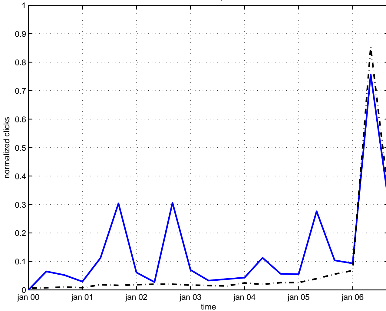
u-duality
