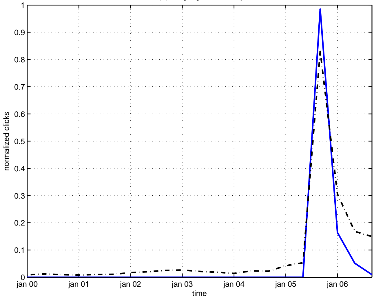
u(n)**m gauge field theory
