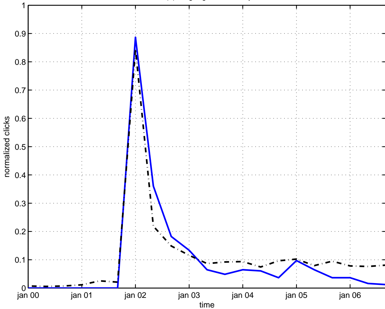
u(n)^3 gauge field theory
