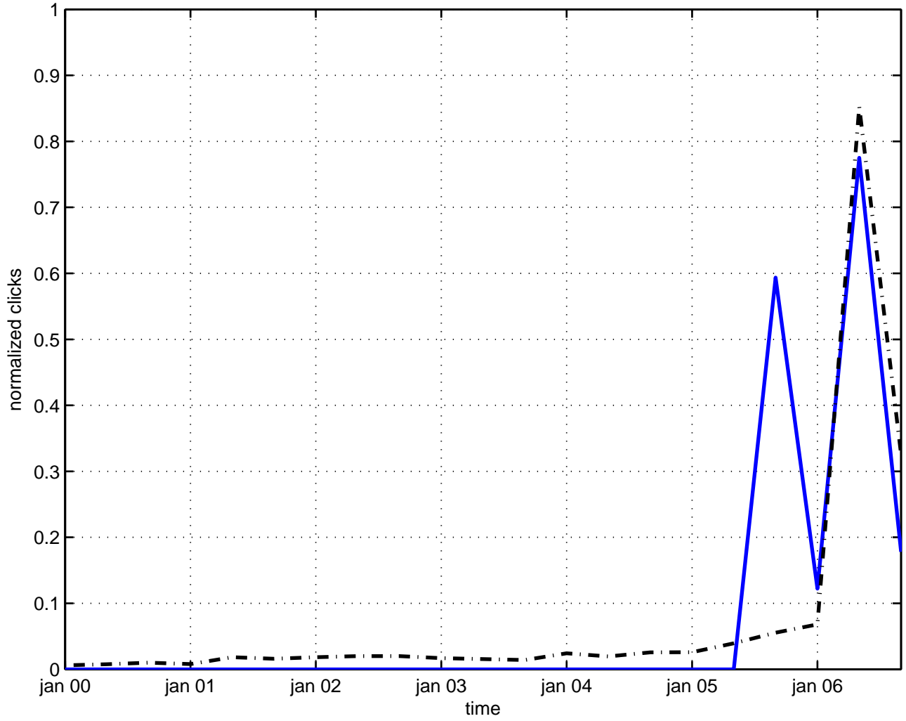
u(n) x u(m) gauge field theory
