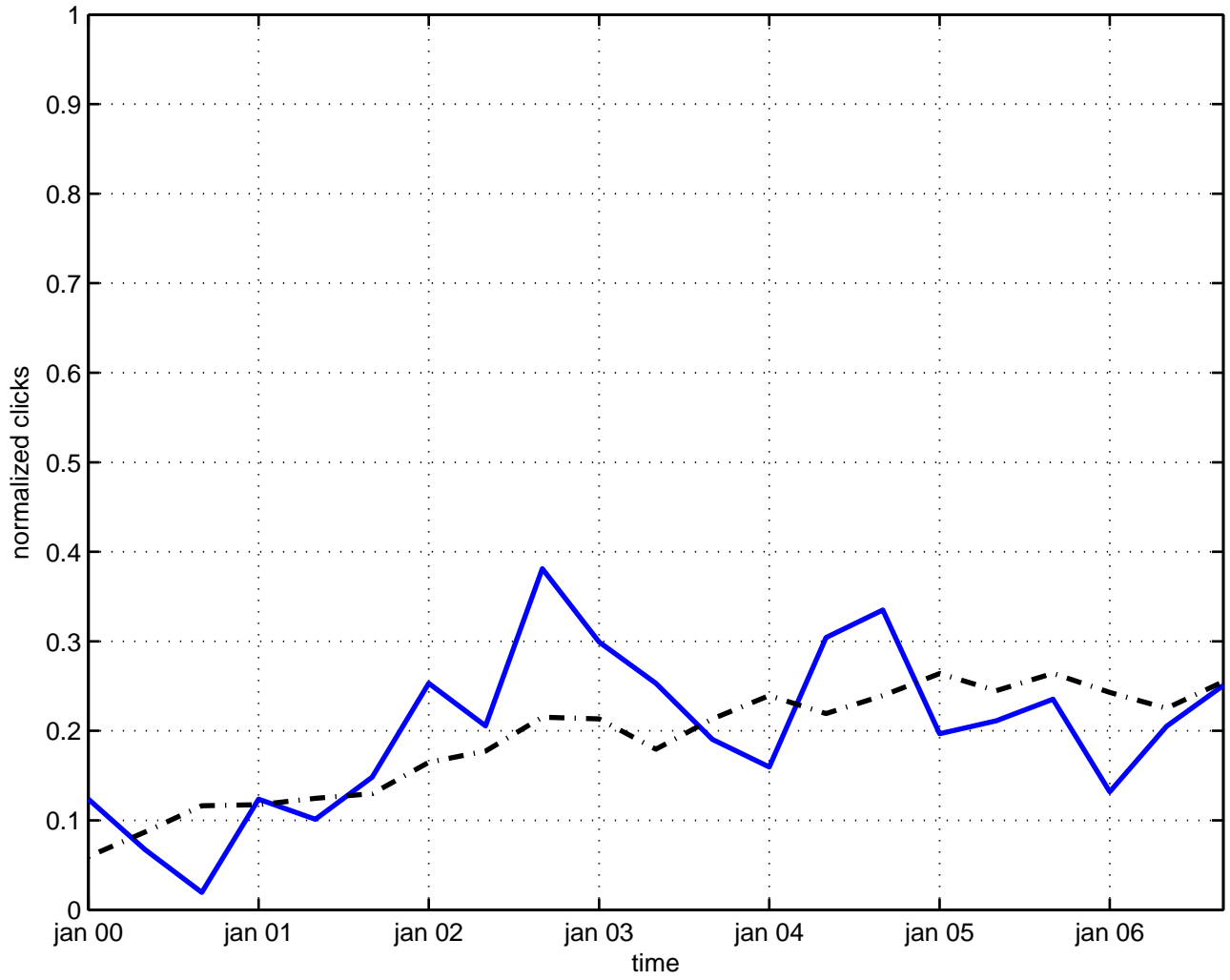
u(n) symmetry
