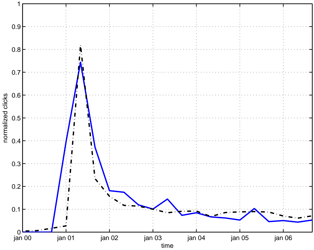
u(n) sigma model
