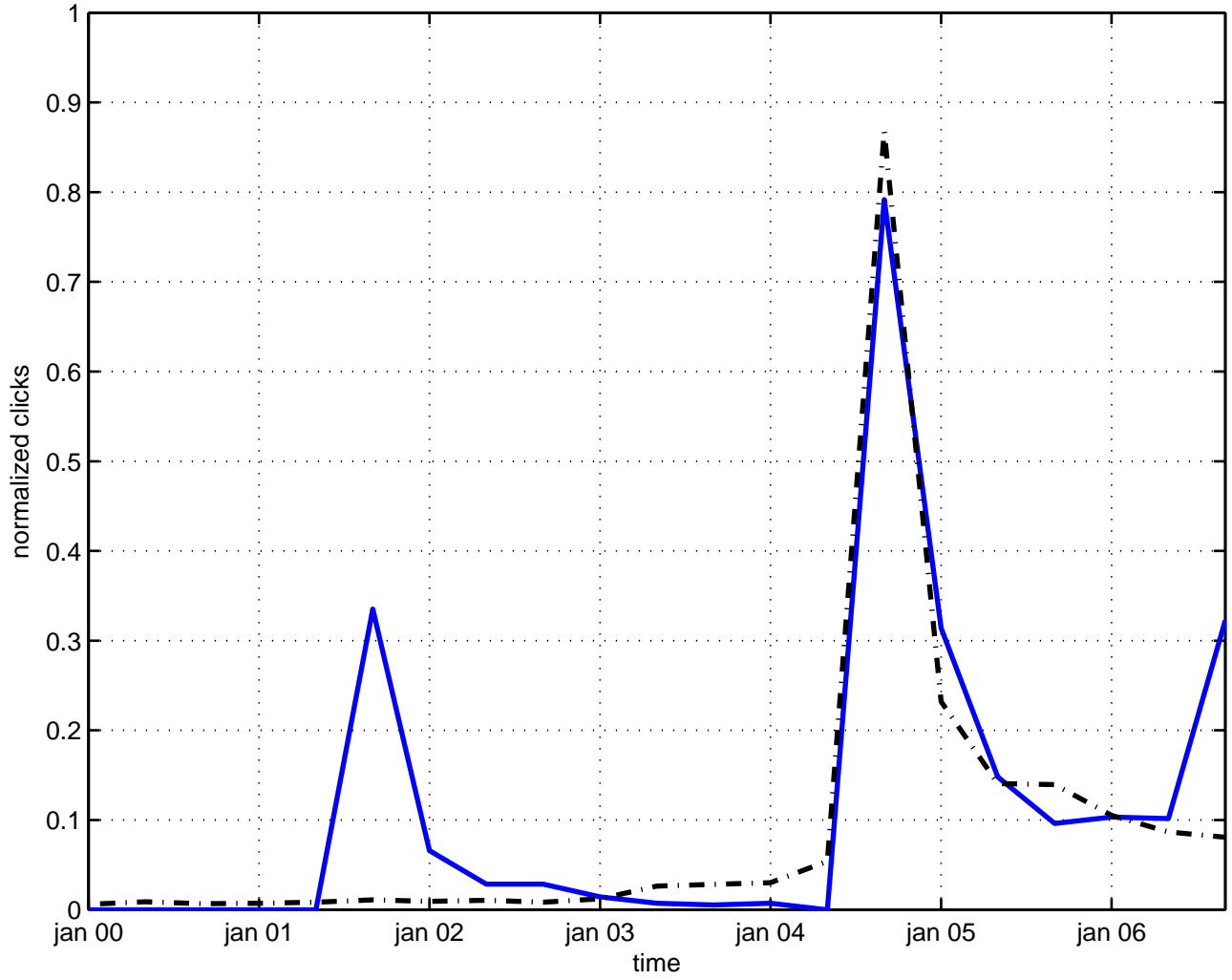
u(n) matrix model
