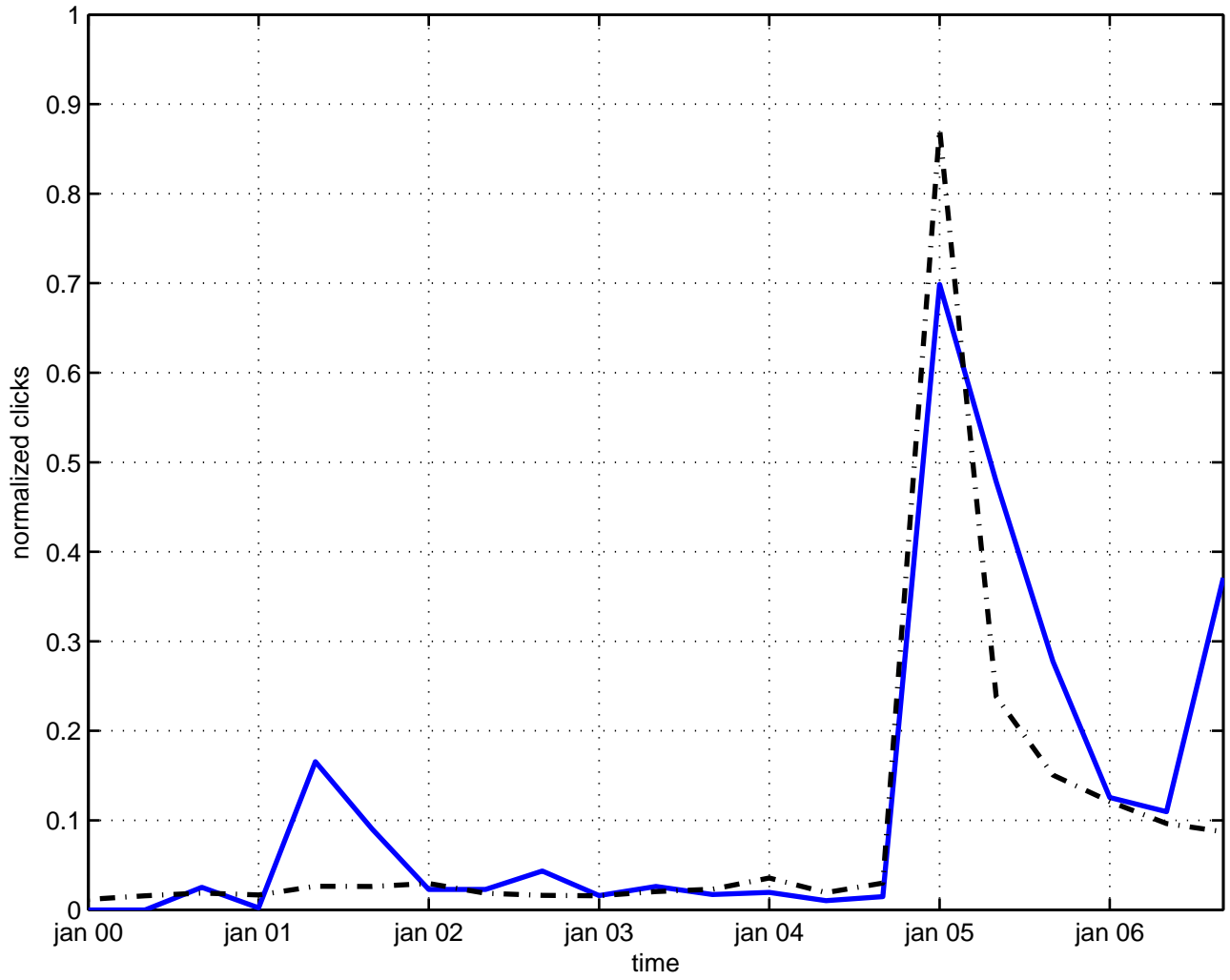
u(n) group theory
