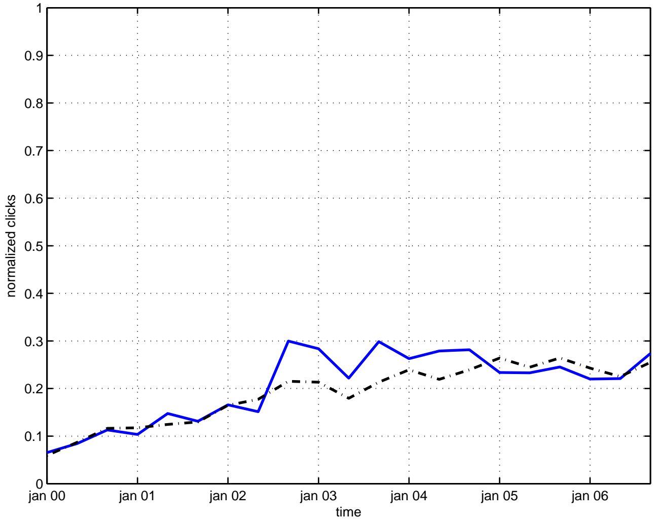
u(n) gauge field theory
