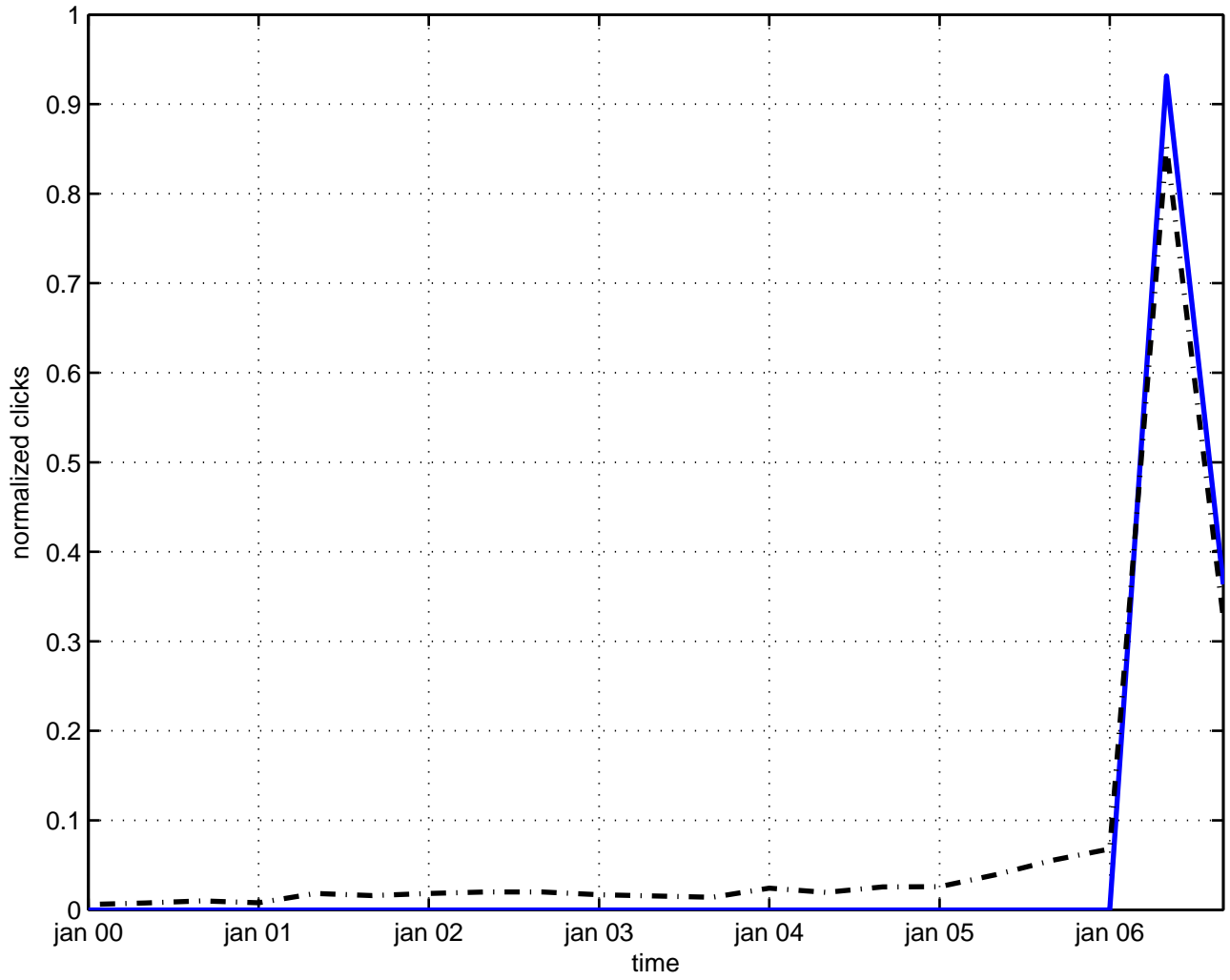
u(n) field theory
