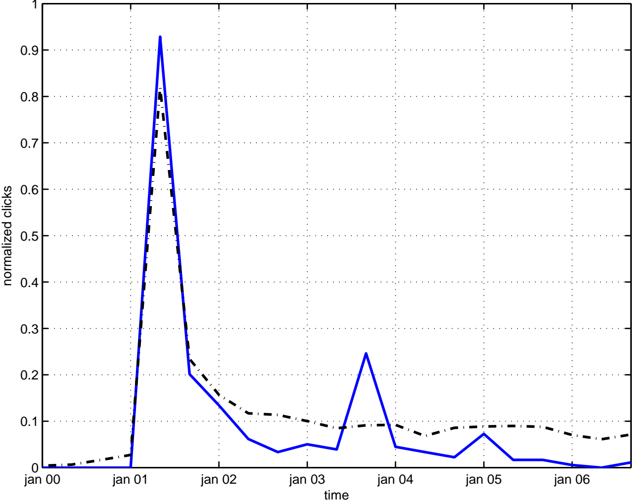
u(infinity) symmetry
